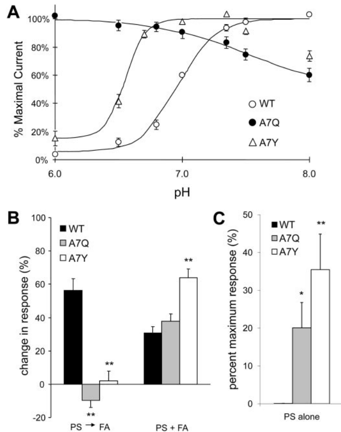
Fig. 8. Altered response of A7Q and A7Y to allosteric modulators. A, proton inhibition curves in the presence of 100 \mu M glycine and 100 \mu M glutamate. WT receptors are highly sensitive to pH modulation, with a pK_a value of 6.97. Decreased proton inhibition was observed in A7Y ( pK_a = 6.59 ), whereas A7Q was insensitive to proton block and inhibited by high pH. Inhibition of A7Y was also seen at high pH values, which were not used in calculating the pK_a for that mutant. B, current potentiation by 100 \mu M PS, applied either before or in the presence of agonist. PS preapplication yielded \sim 50\% potentiation of the WT full agonist response but had little effect on A7Q or A7Y (WT: 56 \pm 7\% ; A7Q: -10 \pm 5\% ; and A7Y: 2 \pm 6\% ). However, concurrent treatment with PS and full agonist restored potentiation in both mutants (WT: 31 \pm 4\% ; A7Q: 38 \pm 4\% ; and A7Y: 64 \pm 5\% ). C, application of 100 \mu M PS was found to partially activate both A7Q and A7Y even in the absence of agonist, whereas having no effect on WT (WT: 0.1 \pm 0.0\% ; A7Q: 16 \pm 6\% ; and A7Y: 30 \pm 10\% ). *, p < 0.05 (significant); **, p < 0.01 (highly significant).
