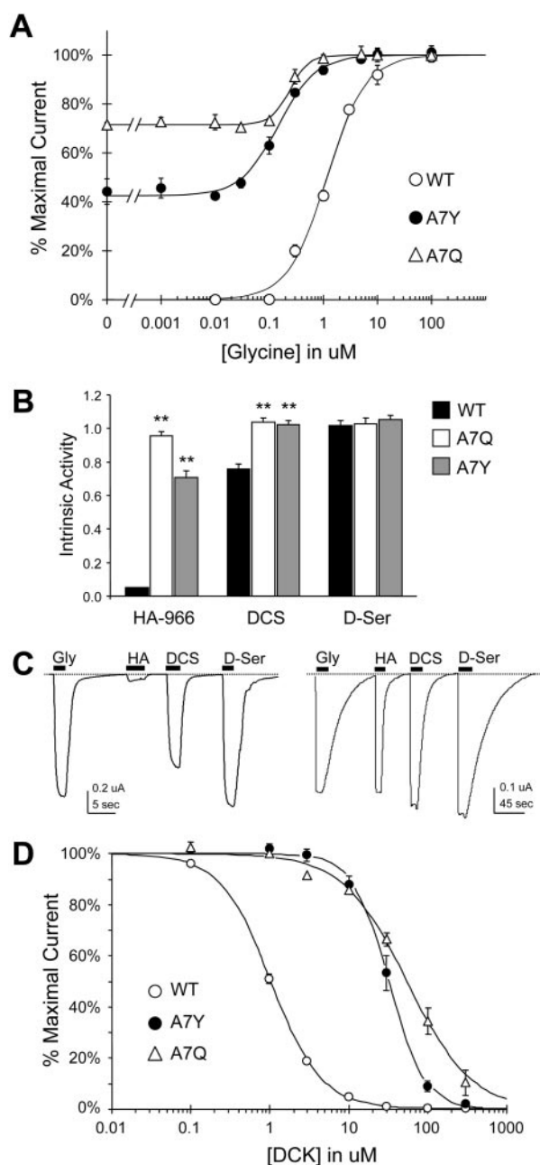
Fig. 2. Altered activation equilibrium in NR1 A7Q and A7Y. A , glycine concentration-response curves in the presence of 100 \mu M L-glutamate. Both A7Q ( \Delta ) and A7Y ( \bullet ) exhibited significant glycine-independent current (71 and 44%, respectively) and increased sensitivity to glycine. Concentration midpoints were 0.24 \mu M for A7Q and 0.15 \mu M for A7Y, compared with 1.16 \mu M for WT. Hill coefficients were 2.5 for A7Q and 1.2 for A7Y, compared with 1.2 for WT. B , response to glycine-site partial agonists, calculated as a fraction of full agonist response. HA-966 (500 \mu M), 1 mM DCS, and 100 \mu M D-serine were coapplied with 100 \mu M glutamate. Both A7Q and A7Y displayed increased activity in response to HA-966 and DCS, but not D-serine. Intrinsic activities for WT, A7Q, and A7Y were as follows: HA-966: 0.05 \pm 0.00 , 0.96 \pm 0.02 , and 0.71 \pm 0.04 ; DCS: 0.76 \pm 0.03 , 1.04 \pm 0.02 , and 1.02 \pm 0.02 ; and D-Ser: 1.02 \pm 0.03 , 1.03 \pm 0.07 , and 1.06 \pm 0.03 . C , representative whole cell traces illustrating the response of WT (left) and A7Q (right) to glycine-site partial agonists in the presence of 100 \mu M glutamate. A7Q receptors exhibit increased partial agonist responses and markedly slow deactivation. D , inhibition by DCK, a competitive glycine-site antagonist, in the presence of 10 \mu M glycine and 100 \mu M glutamate. Both mutants were significantly less sensitive to DCK inhibition. IC_{50} values were 51.5 \mu M for A7Q and 31.7 \mu M for A7Y, compared with 1.04 \mu M for WT. Hill coefficients were 1.1 for A7Q, 2.3 for A7Y, and 1.5 for WT. Calculated K_D values were as follows: A7Q (1.21), A7Y (0.47), and WT (0.11). *, p < 0.05 (significant); **, p < 0.01 (highly significant).
